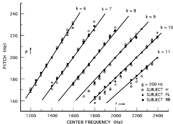
FIG. 2. Experimental data with our predictions superimposed, show pitch as a function of the central frequency f = (k + 1)\omega_0 + \Delta\omega for a three-component complex tone \{f - g, f, f + g\} , for k = 6, 7, 8, 9, 10 , and 11 . The component spacing is g = \omega_0 = 200 Hz. Circles, triangles and dots represent experimental data for three different subjects (from Schouten et al. [4]). The perceived pitch shifts linearly with the detuning \Delta\omega . The pitch-shift effect we predict is shown superimposed on the data as solid lines satisfying the equation P = g + 2[f - (k + 1)g]/(2k + 1) . The lines describe the behavior of the response frequency in a three-frequency resonance formed with the two lowest-frequency components of the stimulus. The lines agree with the psychophysical data without any fitting parameters.
